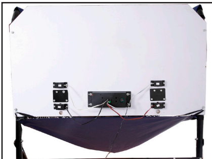
LED infrared dual display electronic scoring and timing clock -- 9" x 3.25". Motion sensors mounted above and below rim -- 3" x 1.25" each.
