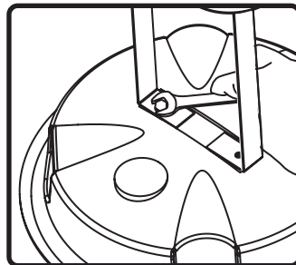
2. Attach in-ground/security brackets to speaker base using stainless steel bolts.
