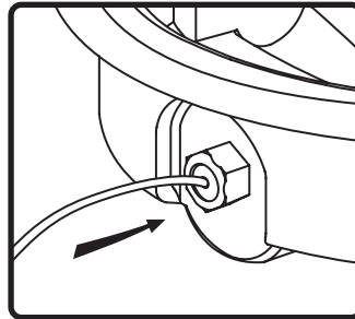
3. Thread signal wire thru liquid-tight strain relief and tighten seal.
