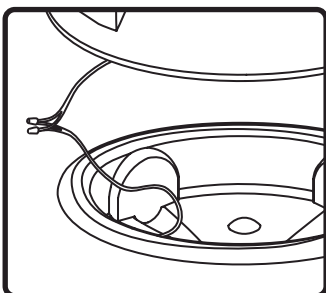
5. Attach signal wire to wire leads. Use wire nuts provided. For added water-proofing, grease caps are recommended.
