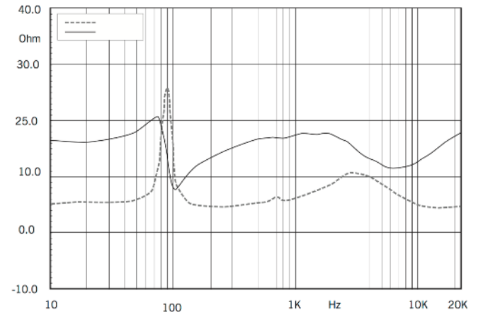
Phase/Impedance Response
