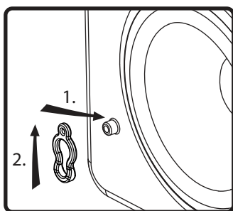
4. Attach grille safety clip by placing the large end of the clip over snap-fit post (1), then sliding clip until small end snaps into place around post (2).
