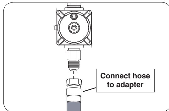
Fig. 3-4 Install quick connect hose
