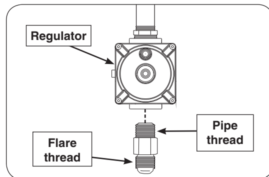
Fig. 3-2 Install adapter to regulator
